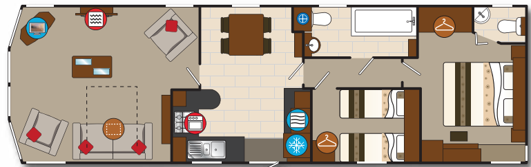
38 X 12' 6" 2 BEDROOM SLEEPS 6
